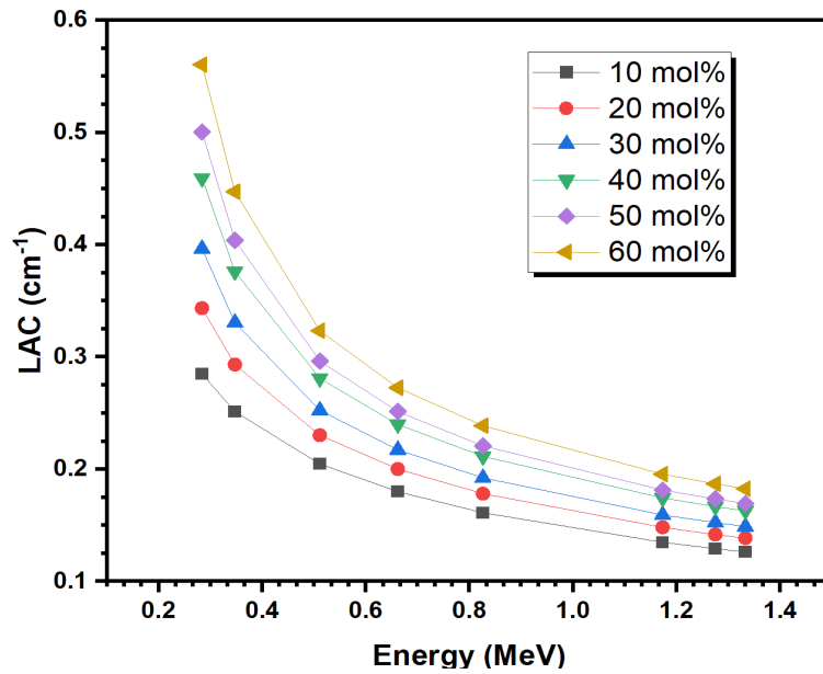
Fig. 8. The linear attenuation coefficient (LAC) against energy of (80-x)\text{B}_2\text{O}_3-x\text{TeO}_2-10\text{Li}_2\text{O}-10\text{Al}_2\text{O}_3 ( x=10-60 mol%) glass samples.
