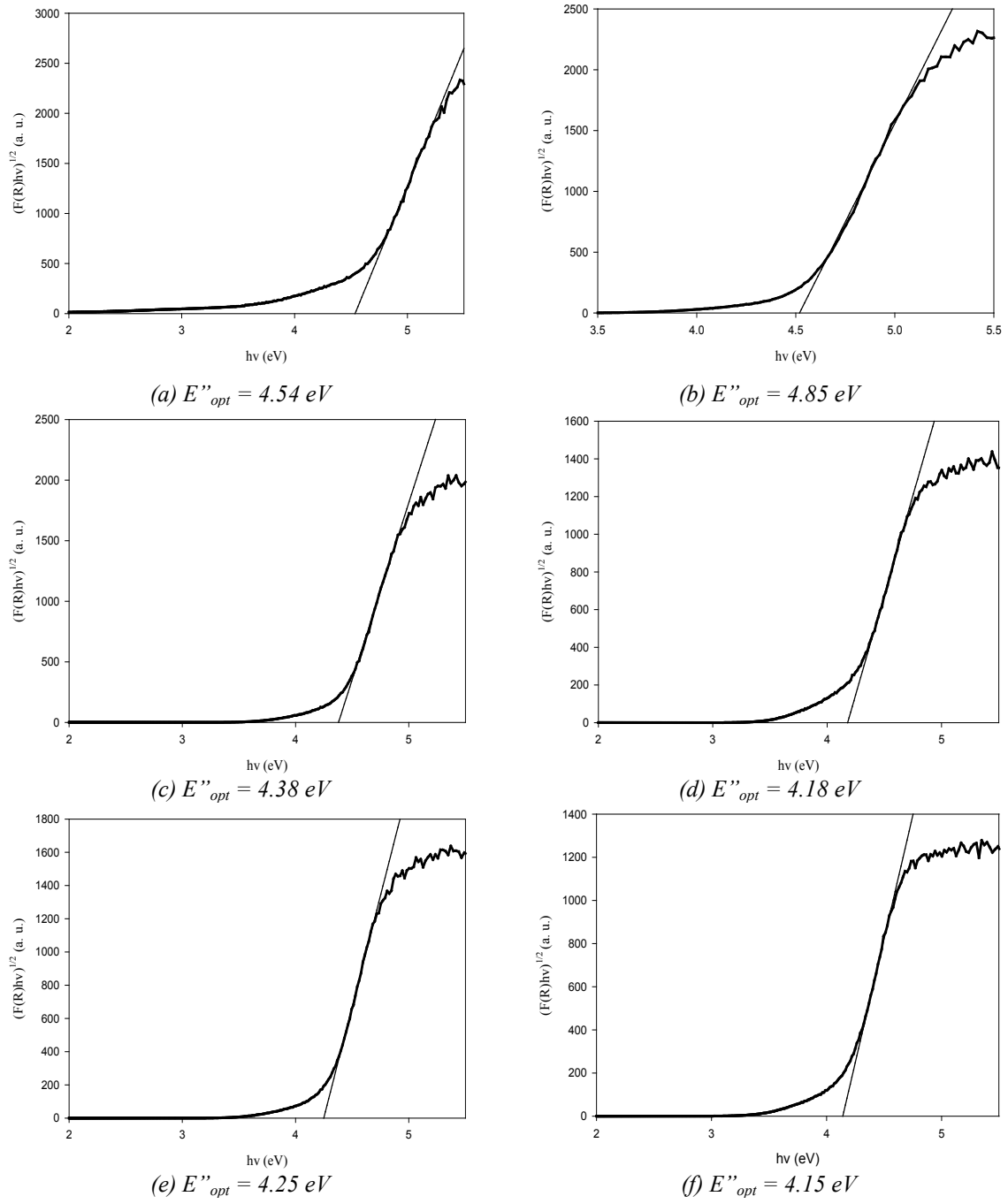
Fig. 3. Plots of (ahv)^{1/2} against (hv) of (80-x)B_2O_3-xTeO_2-10Li_2O-10Al_2O_3 ( x=10-60 mol% for (a) to (f), respectively) glass samples.
