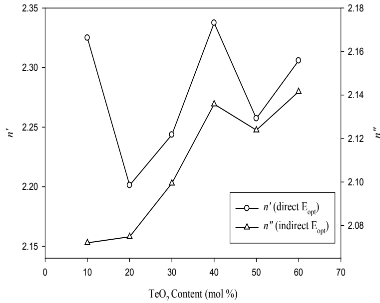
Fig. 5. Plots of direct, n' and indirect, n'' allowed E_{opt} based- n with TeO_2 content for (80-x)B_2O_3-xTeO_2-10Li_2O-10Al_2O_3 ( x = 10-60 mol%) glass samples.
