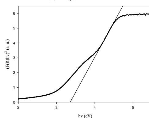
(f) E'_{opt} = 3.36 \text{ eV}
