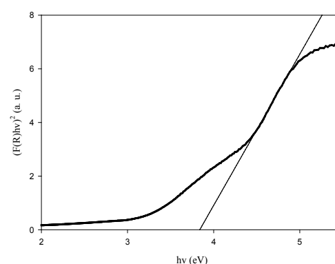
(b) E'_{opt} = 3.84 \text{ eV}
