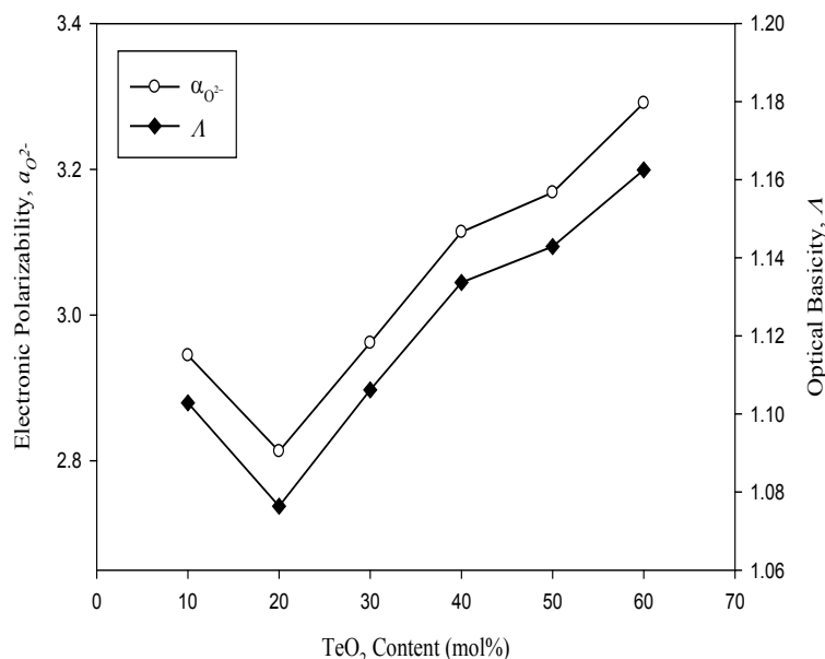
Fig. 7. Plot of \alpha_{O^{2-}} and \Lambda with \text{TeO}_2 content of (80-x)\text{B}_2\text{O}_3-x\text{TeO}_2-10\text{Li}_2\text{O}-10\text{Al}_2\text{O}_3 ( x=10-60 mol%) glass samples.
