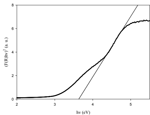
(c) E'_{opt} = 3.64 \text{ eV}
