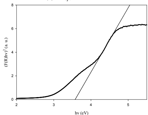
(e) E'_{opt} = 3.58 \text{ eV}
