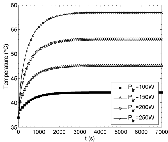
Figure 7: Temperature variation at origin for various laser power settings
