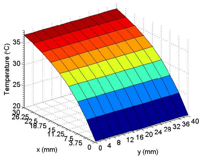
Figure 9: Steady state temperature distribution without laser
