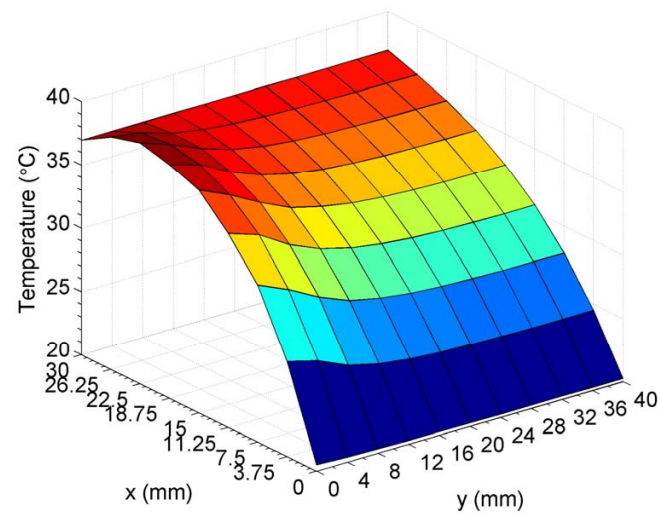
Figure 10: Steady state temperature distribution with laser
