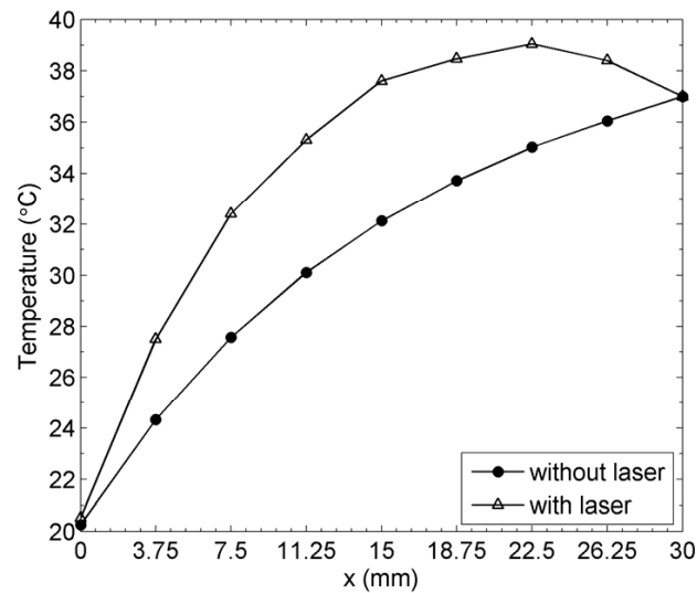
Figure 8: Steady temperature variation at origin for laser
