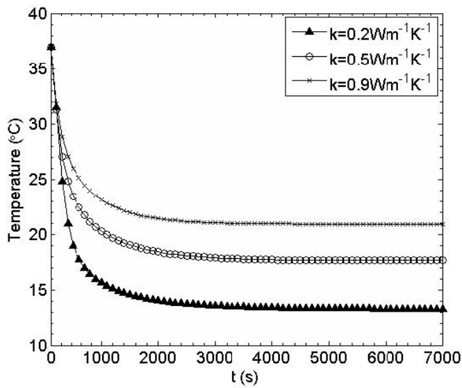
Figure 6: Surface temperature variation for various heat conductivities
