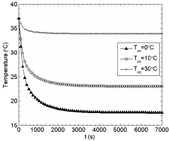
Figure 5: Surface temperature variation for various ambient temperatures
