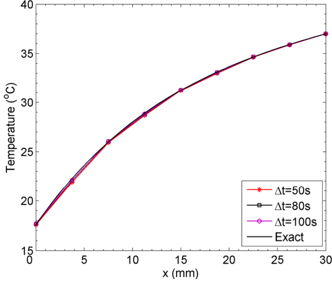
Figure 2: Steady-state temperature distribution along the x axis
