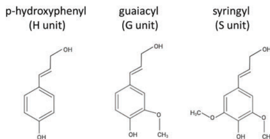
Figure 3: Lignin unit molecular structure
