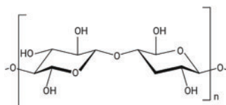
Figure 1: Cellobiose structure, monomer of cellulose
