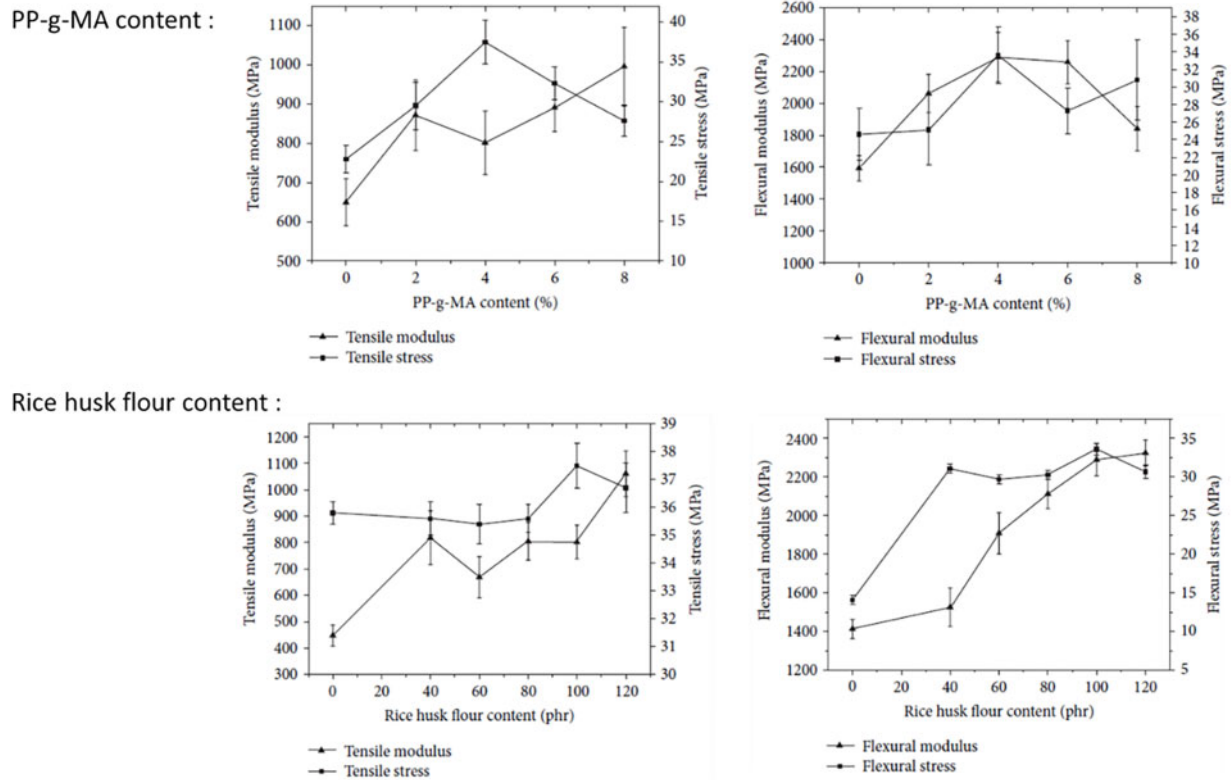
Figure 9: Mechanical properties and the content of PP-g-MA and RH fibers—Extracted from Tran et al. [120]
