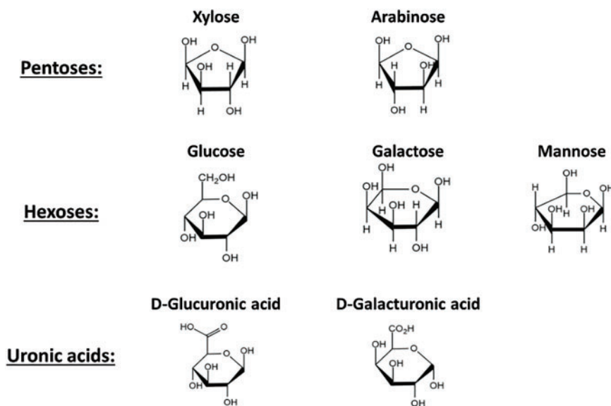
Figure 2: The monomers of hemicelluloses
