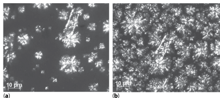
Figure 6 Optical microscopy observations on P(EV-co-RA)-50/50 sample at T=100\text{ }^{\circ}\text{C} (a) and T=75\text{ }^{\circ}\text{C} (b) during cooling from the melt.
