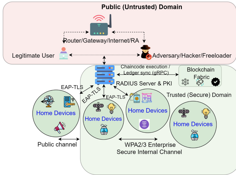
Figure 1: Proposed blockchain-centric SH network architecture.
