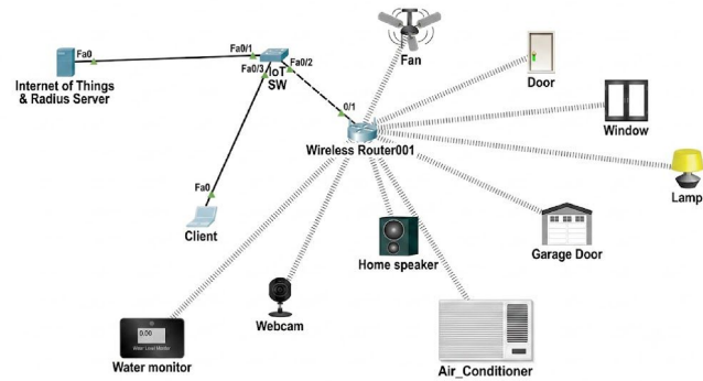
Figure 6: Simulated nine-device smart home network.
