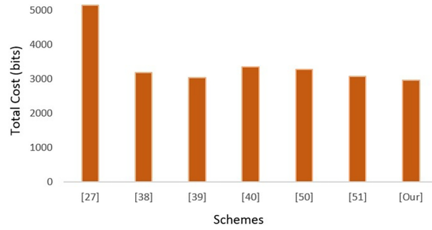
Figure 8: Total communication cost (bits) across schemes [27,38–40,50,51].
