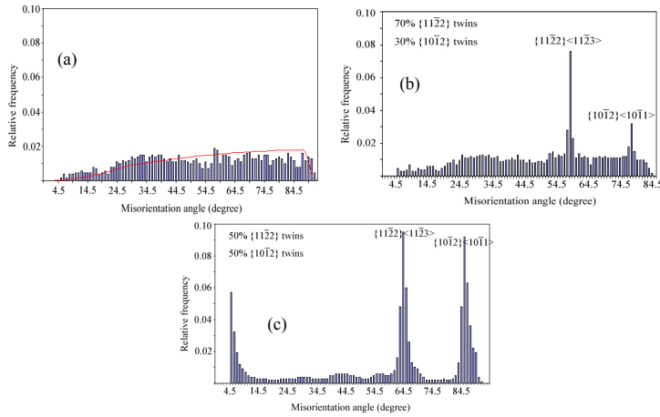
Figure 4: Misorientation-angle distributions of samples deformed to 0% (a), 10% (b) and 20% (c) reduction.
