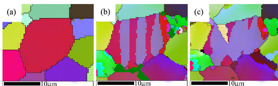
Figure 6: Initial grain with c axis close to the ND (dark red) (a); 10% deformation: \{11\bar{2}2\} compression twins outlined by red lines (b); 20% deformation: a part of \{11\bar{2}2\} twins undergoes secondary \{10\bar{1}2\} tension twinning, (c). outlined by blue twinning boundaries delimiting the tension twin (in yellow colour).
