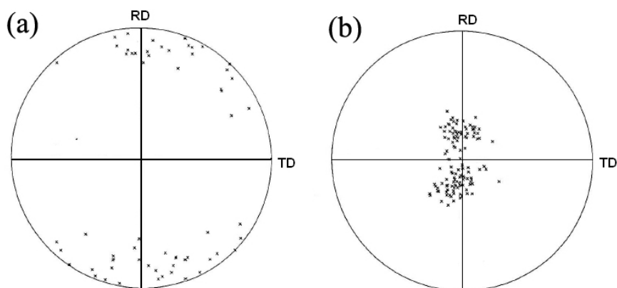
Figure 8: Initial \{0002\} -Pole figure of grains having \{10\bar{1}2\} twin (a) and Initial \{0002\} -Pole Figure of grains having \{11\bar{2}2\} twin (b) after 10% deformation.
