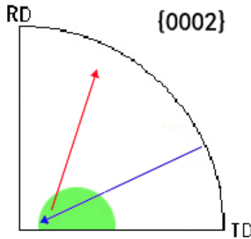
Figure 10: Schematic reorientation of c axes by \{10\bar{1}2\} twinning (blue) and \{11\bar{2}2\} twinning (red arrow).
