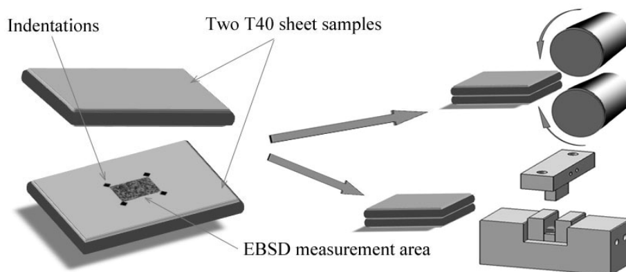
Figure 1: The preparation of samples and arrangement of the rolling and channel die compression tests
