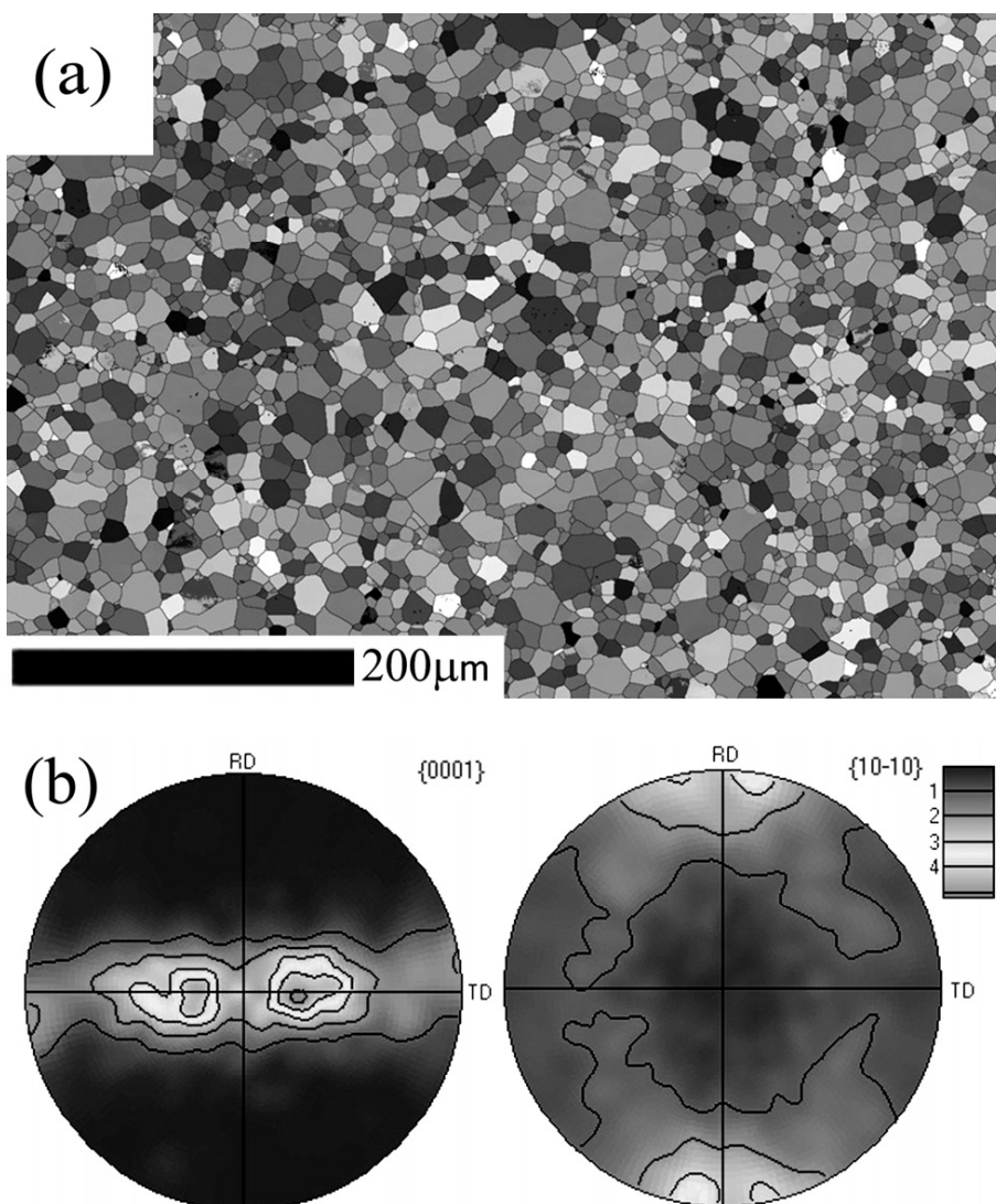
Figure 2: EBSD orientation mapping (a) and 0002, pole figures (b).
