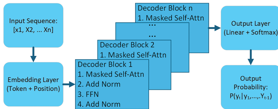
Figure 5: Decoder-only model architecture schematic
