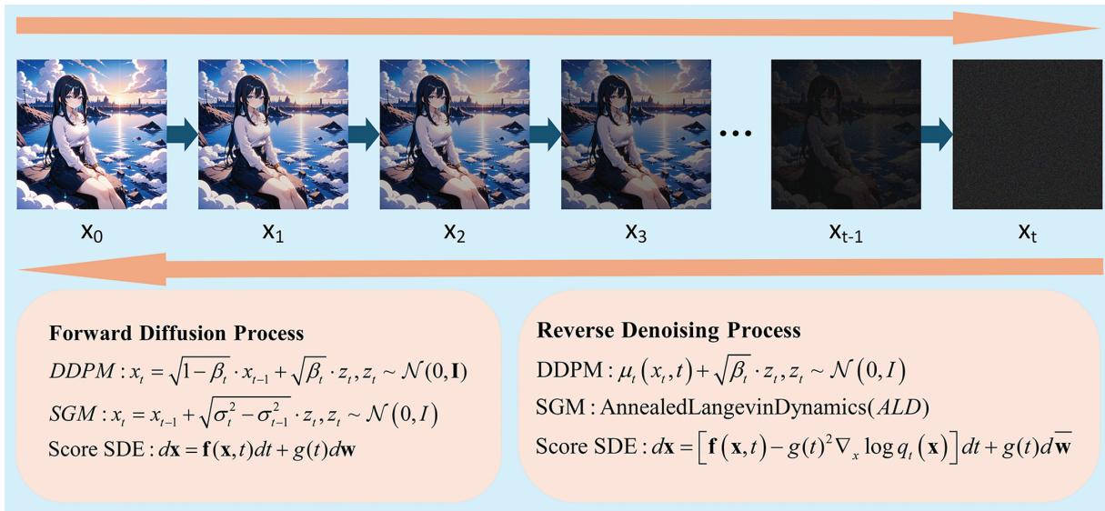
Figure 2: Overview of diffusion models (DDPM, SGM, and Score SDE diffusion and denoising processes)
