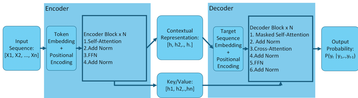
Figure 4: Encoder-decoder model architecture diagram
